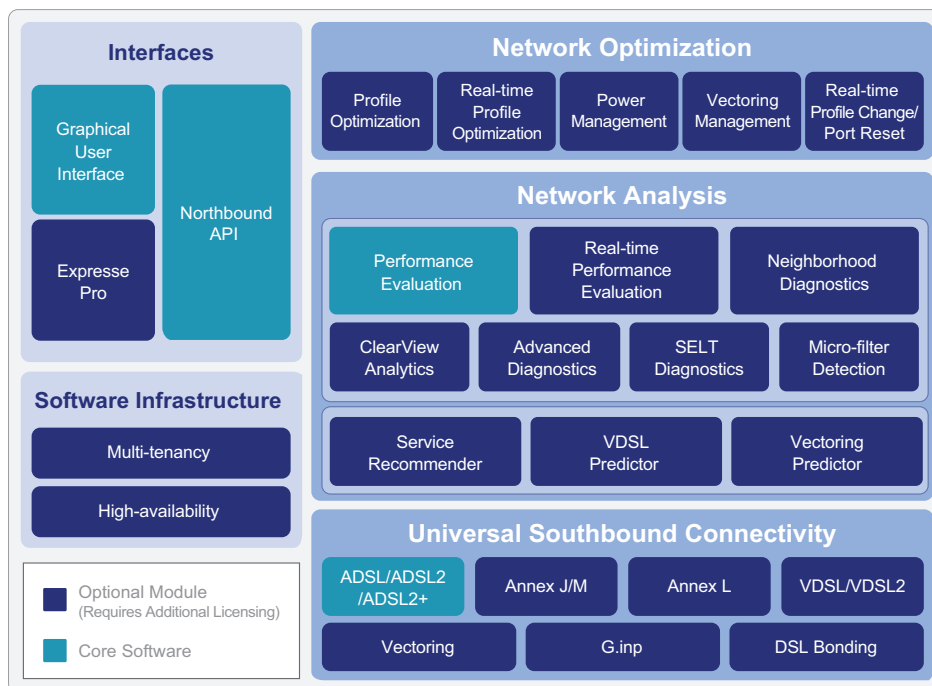
FIGURE 2. ASSIA Express Software Architecture with prerequisites for ASSIA Power Management module – PE license + PO license + at least one type of access
