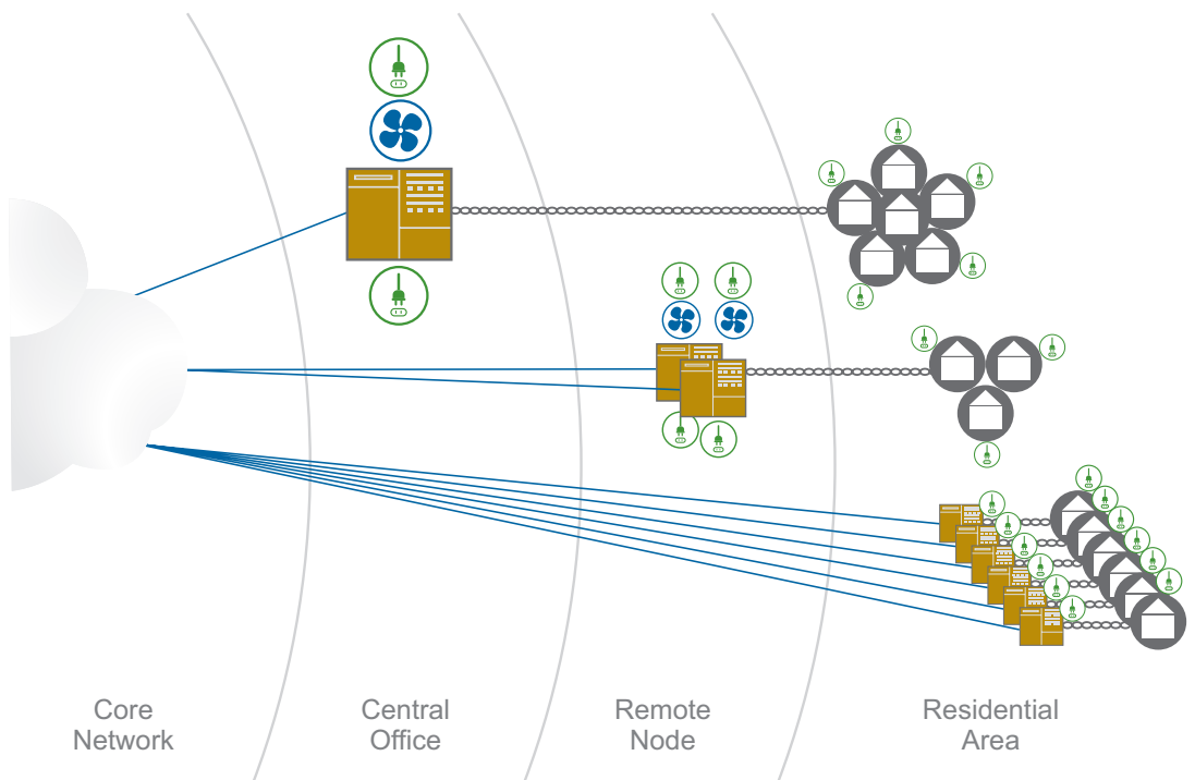
FIGURE 1. The Power Hungry DSL Transmission Chain
